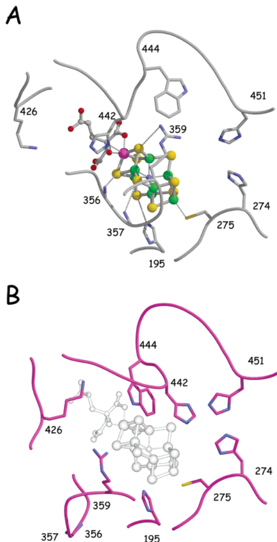
Figure 5. Protein environment of MoFe protein (A) and apo-MoFe protein (B) in the vicinity of the FeMo-cofactor binding area. Parts of the C _{\alpha} backbone and important side-chain residues in the \alpha -subunit are shown. FeMo-cofactor is represented by a ball-and-stick model. Gray dotted lines indicate hydrogen-bonding interactions between the residues and the FeMo-cofactor. The theoretical position of FeMo-cofactor in apo-MoFe protein is indicated in light gray after superposition of the C _{\alpha} positions of the \alpha -subunits in apo-MoFe protein and MoFe protein. The following key residues for FeMo cofactor insertion are shown: (1) \alpha -His 274 , \alpha -His 442 , \alpha -His 451 (“His triad” in apo-MoFe protein); (2) \alpha -Trp 444 (part of the FeMo-cofactor “lock”); (3) \alpha -355 through \alpha -359 (part of the “lid” loop from \alpha -353 through \alpha -364); and (4) \alpha -Lys 426 (“anchor” for the homocitrate of the FeMo-cofactor). Programs MOLSCRIPT 16 and RASTER3D 17 were used to prepare the figure. Atoms are colored the same as those described earlier.
